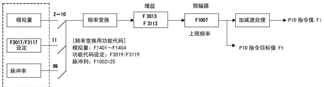
PID 指令值输入切换 F3001/F3101
